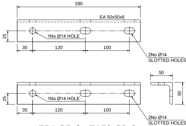
TPA-BR-2 - EA50x50x6 Scale 1:5
