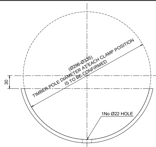
TPC-A-3 - 100x8mm PLATE Scale 1:5
